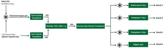
Figure 1. Block diagram detailing the complete signal modeling and recovery.
